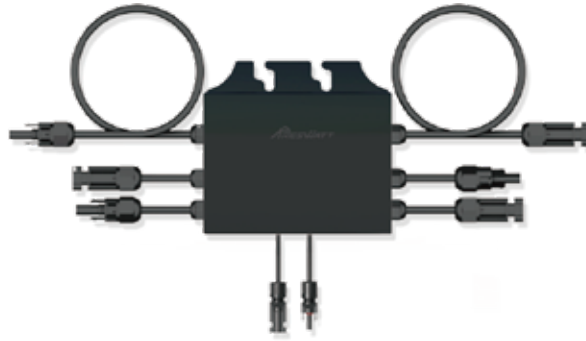
1 to 6 Rapid Shutdown Device
